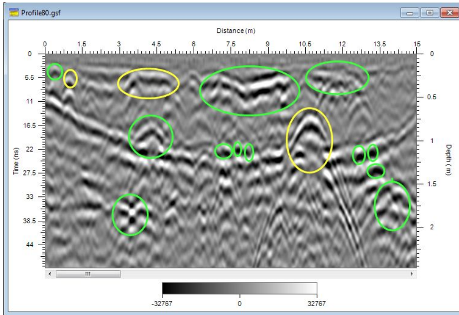
Normal gained data processed and interpreted
