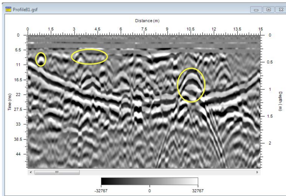
Over-gained data processed and interpreted
